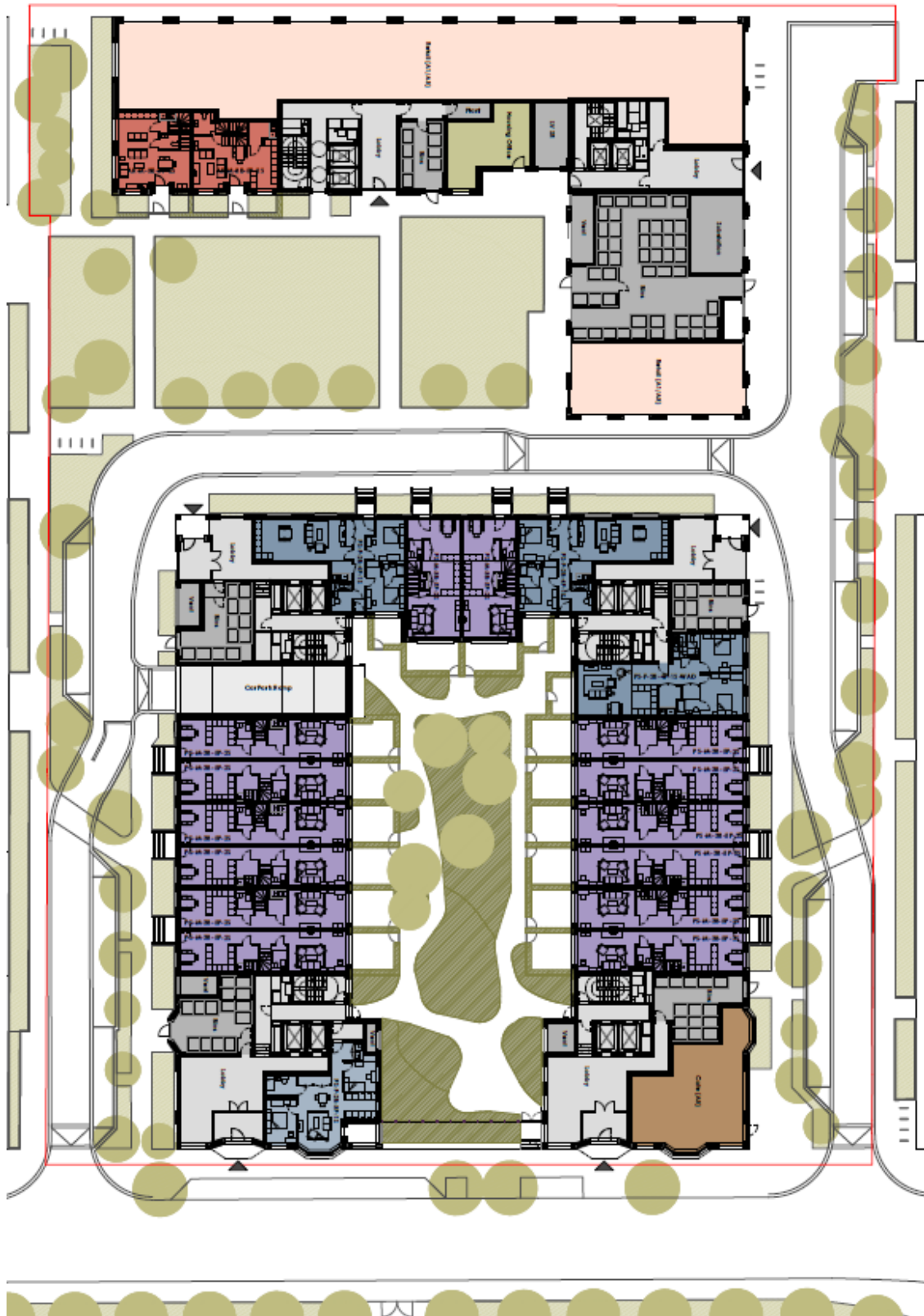
IMAGE 3 - Proposed Ground Floor Plan
